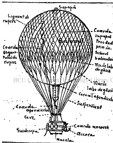
Fig. 2. — Balon liber.
