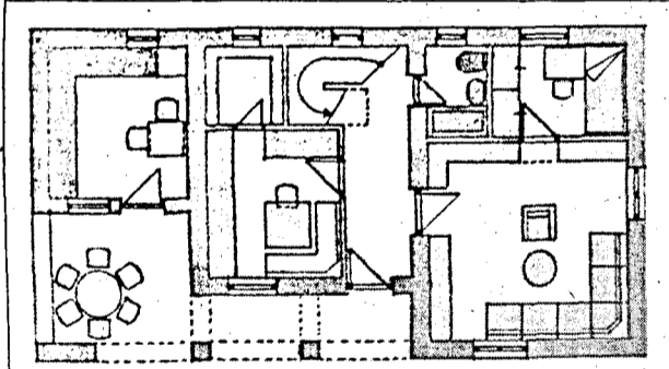
plan parter - varianta 1
