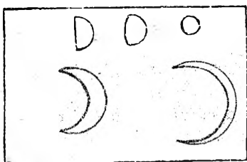
BCU Cluj / Central University Library Cluj Fig. 6. — Fazele lui Venus.
