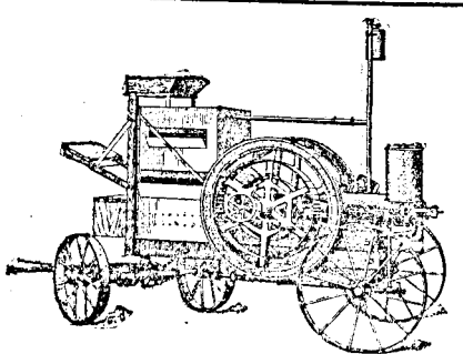
Benzin-Lokomobil.
